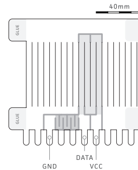
Button design schematic for PASCO paper.
