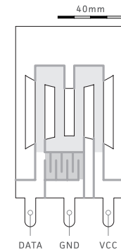
Hinge design schematic for PASCO paper.
