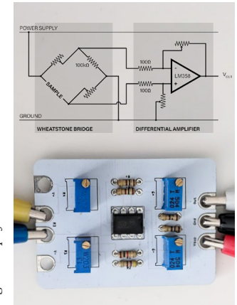
Signal amplifier tool and schematic.
