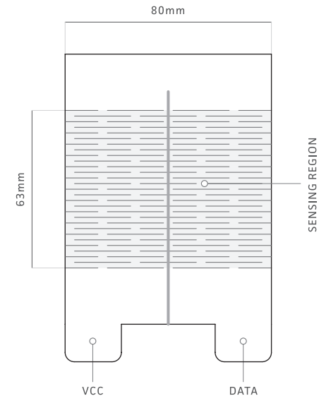
Schematic of fishnet pattern tested
