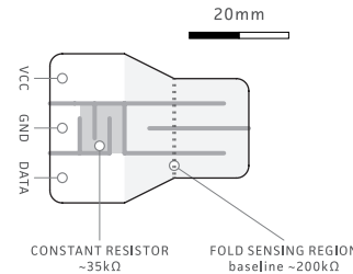
Fold sensor schematic
