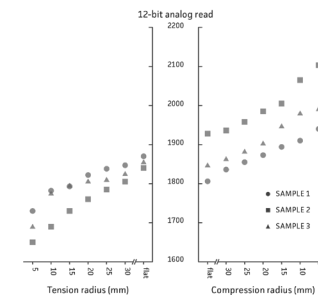
Bend sensor chart
