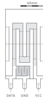
Hinge design schematic for SF paper.
