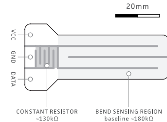
Bend sensor schematic
