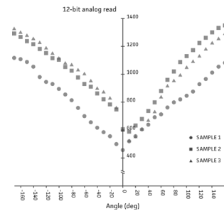
Fold sensor chart
