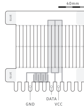
Button design schematic for SF paper.
