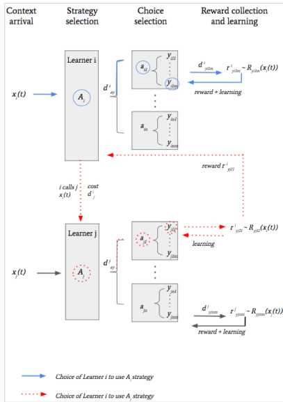
Figure 2: Structure of the Hierarchical Cooperative Contextual Bandit
