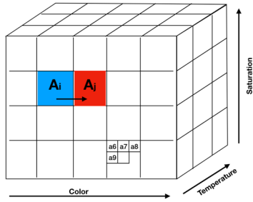
Figure 3: Simplification of the creative space and moving from strategy A_i to A_j
